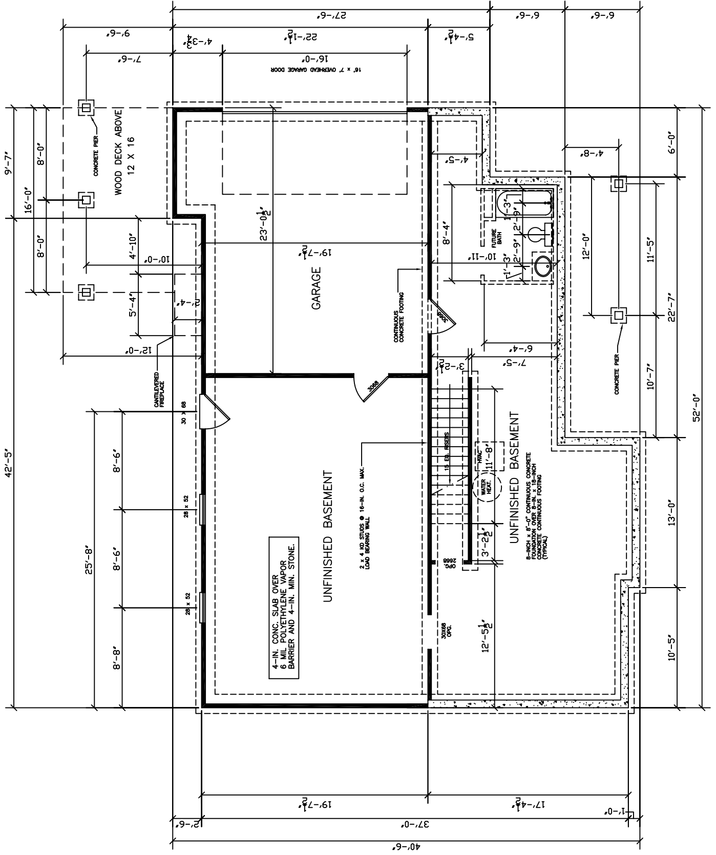
BASEMENT FOUNDATION PLAN
